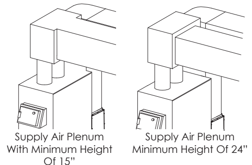
Supply Air (Hot Air) Duct Work Outlet Size
