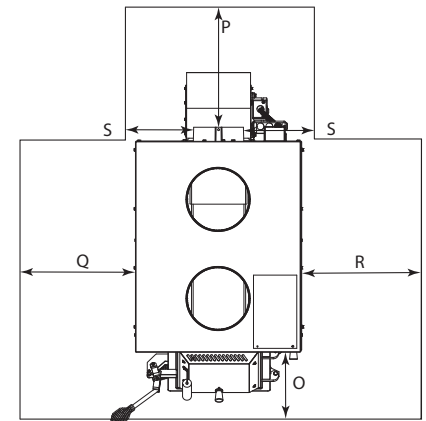
FLOOR PROTECTOR REQUIREMENTS
