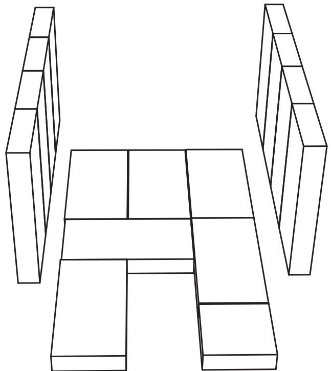
Proper Fire Brick Alignment
