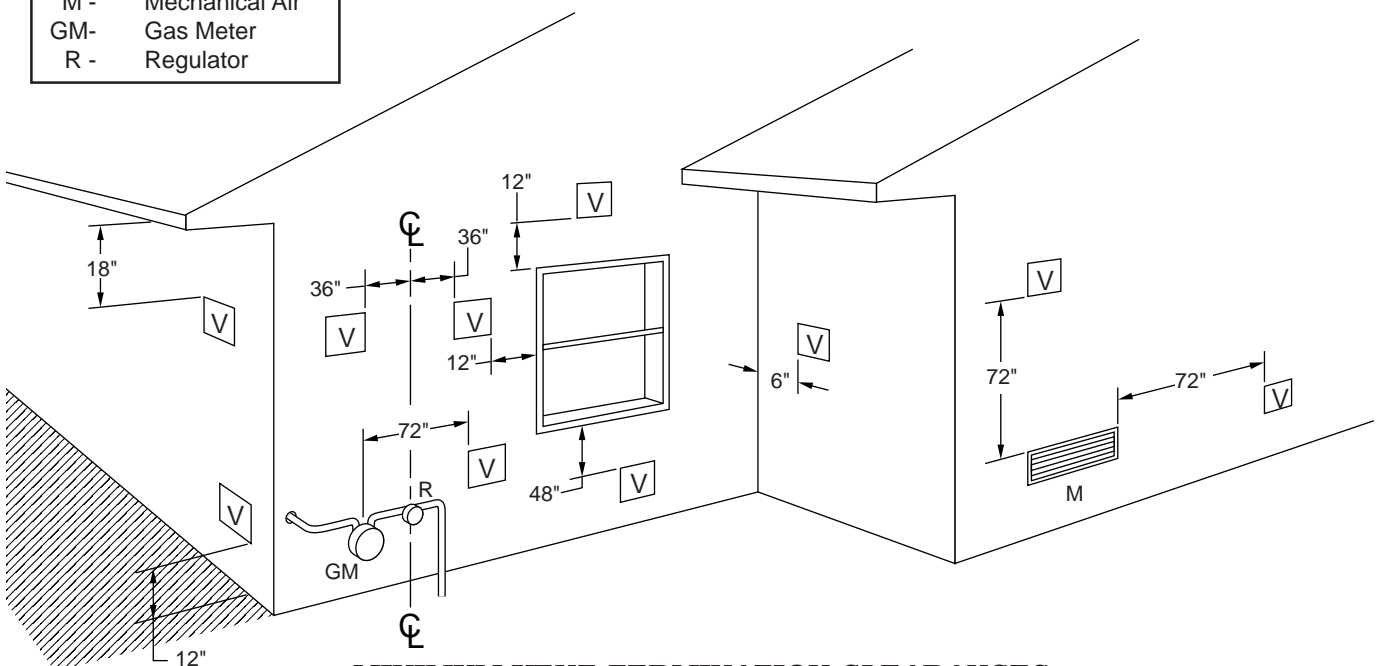
MINIMUM VENT TERMINATION CLEARANCES From combustibles exterior surfaces, gas meter, air intakes, etc.
